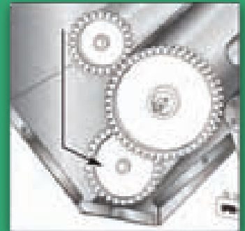
Gear driven rollers provide consistent, even distribution of paste roll after roll.
